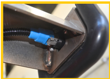
■ Plug and play wiring loom using double O-ring sealed Deutsch plugs.
